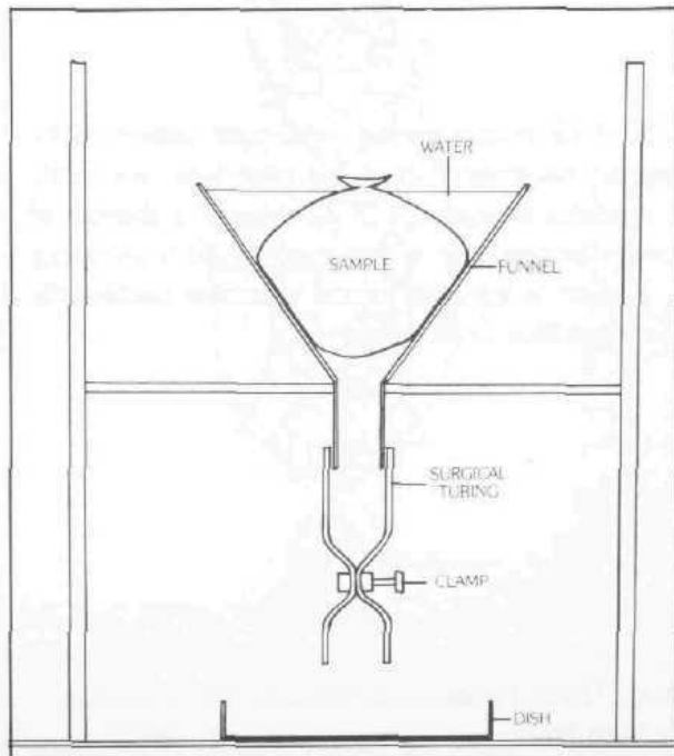
Figure 237 Nematode testing apparatus. Sample is wrapped in gauze and submerged in a water filled funnel. After twenty-four hours, a small amount of water is drawn off and examined with a magnifying lens or dissecting scope.
