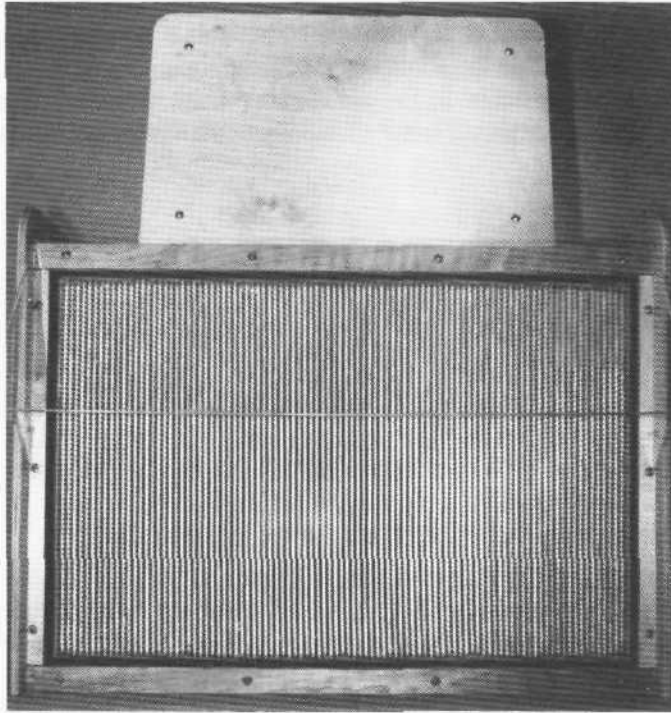
Figure 240 A commercially available laminar flow hood.
